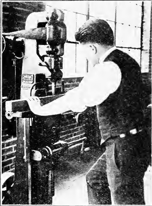
FIG. 195. OPERATING VERTICAL HOLLOW CHISEL MORTISER.
